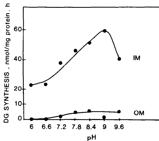
Fig.2. Effect of pH on the rate of endogenous phosphatidic acid hydrolysis by isolated membrane fractions enriched in outer or inner envelope membranes, respectively, from spinach chloroplasts. Assay conditions are described in section 2. The amount of [ ^{14}C ]diacylglycerol at zero time of the incubation was subtracted from all other values. For abbreviations, see fig.1.
